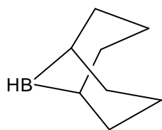
9-BBN
